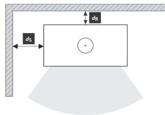
Fig. 3 Safe distances from nonflammable materials
