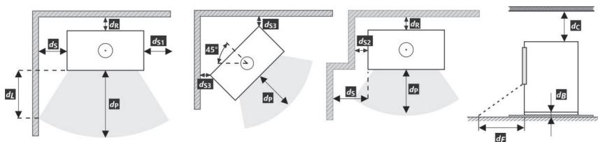
Fig. 2 Safe distances from flammable materials
